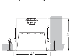
Recessed Spackle Flange
