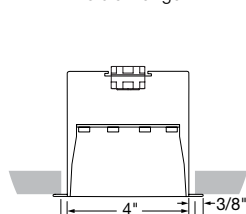
Recessed Visible Flange
