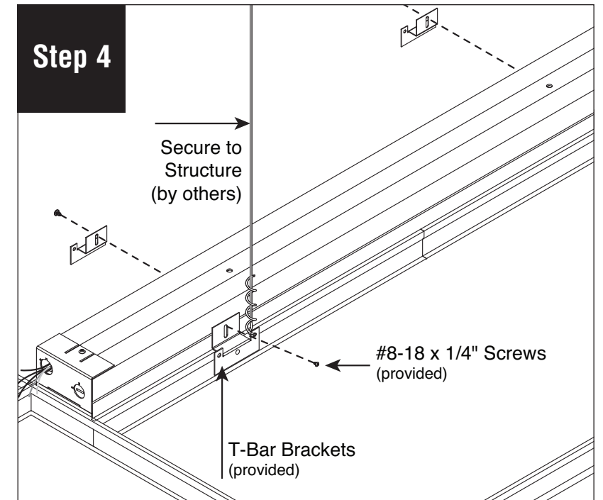
Install T-Bar bracket onto luminaire. Secure with #8-18 x 1/4" screws (provided). Secure luminaire to building structure using tie-wire, as per code.
