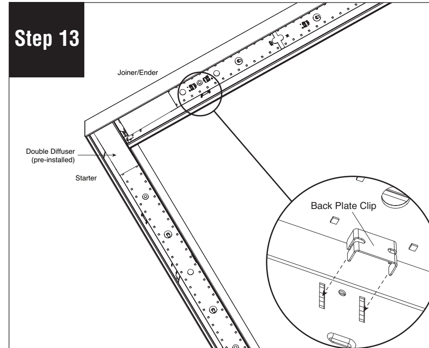
Replace back plates by holding them in their original position and pushing the clips back in. Make sure wire connections are not pinched. (If 1 ft. back plate assembly is near joint, reconnect feed harness to LED board).
