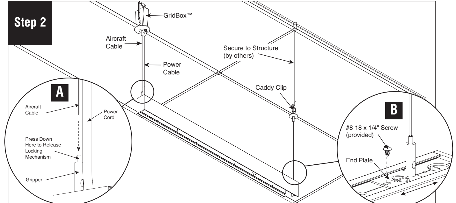
Install GridBox™ and caddy clip onto ceiling grid, then canopies and aircraft cable assemblies. A. Align aircraft cables to grippers and insert on both ends of the luminaire. Adjust pendant to proper height and level. Press down on top of gripper to release locking mechanism if needed. Secure luminaire to structure using tie-wire (by others) according to code. B. End plates are adjustable for custom mounting locations. Remove #8-18 x 1/4" screw (provided) from end plate, then slide end plate to desired location and reinstall #8-18 x 1/4" screw.
