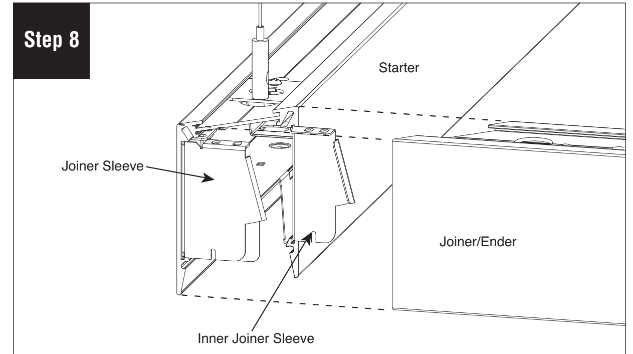
Align starter and joiner/ender, then slide luminaires together.
