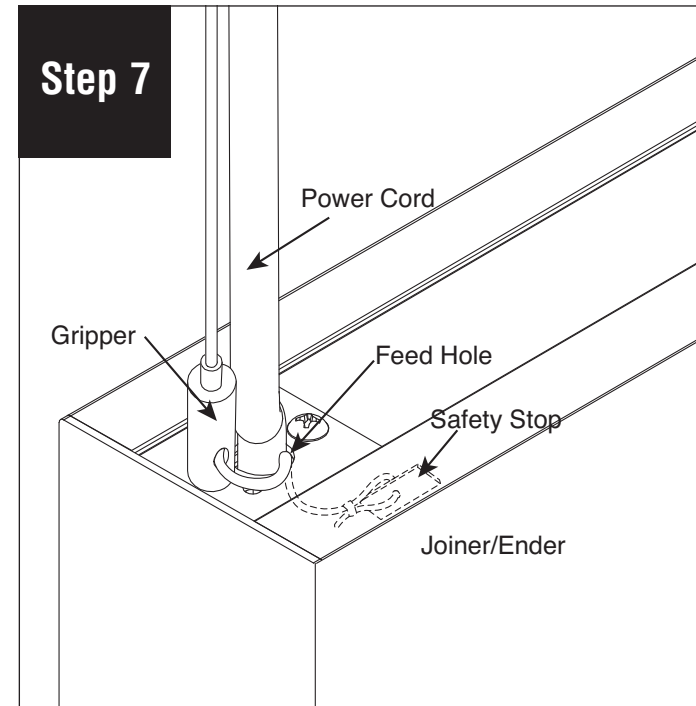
Slide safety stop and safety crimp up to the aircraft cable within 9" of cable gripper. Trim excess cable and insert safety bar assembly through feed hole.
