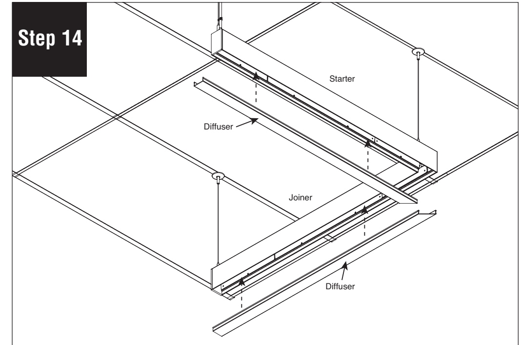
Reinstall diffuser and turn power on to luminaire.
