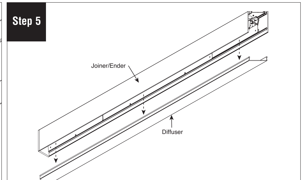
Remove diffuser from joiner/ender and set aside to prevent it from getting dirty or damaged.
