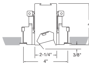
Tech Zone 4" (TZ4 C2T)
