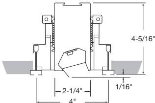
Tech Zone 4" (TZ4 C3)
