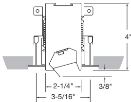
1" Tegular (C1T)
