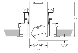
Tech Zone 4" (TZ4 C2)
