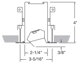
1" T-Bar (C1)
