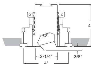
Tech Zone 4" (TZ4 C3F)
