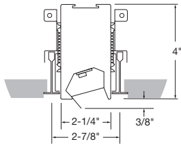
9/16" Tegular (C2T)
