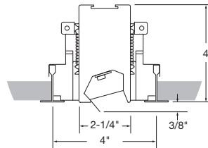
Tech Zone 4" (TZ4 C1)
