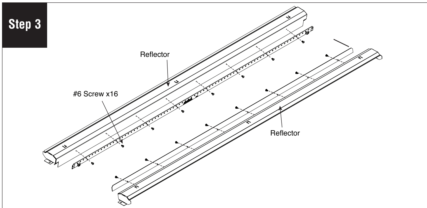
Remove #6 screws holding LED boards onto reflectors and replace boards.
