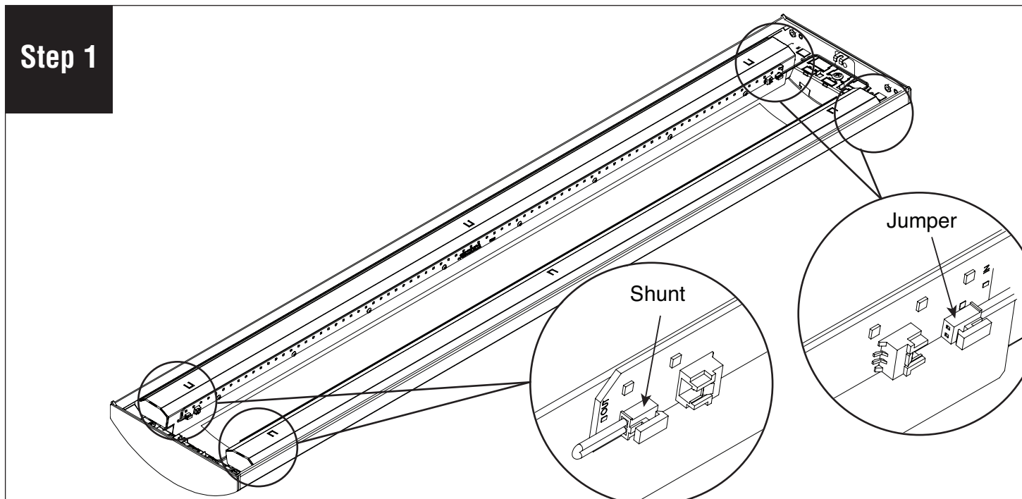
Disconnect all wiring harness. Keep the jumper cable and re-use with new LED engine.
