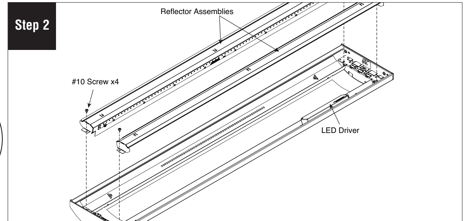
Remove #10 screws on both ends of reflector assemblies then remove the assemblies.
