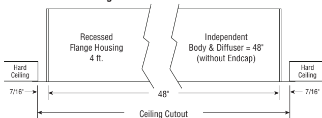
Visible Flange
