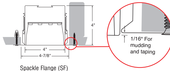
Spackle Flange (SF)
