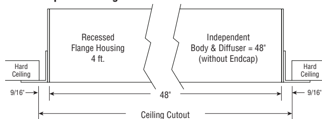
Spackle Flange
