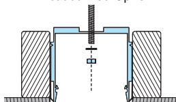
Screw Mount Option
