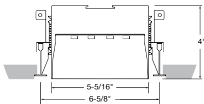
9/16" Tegular (C2T)
