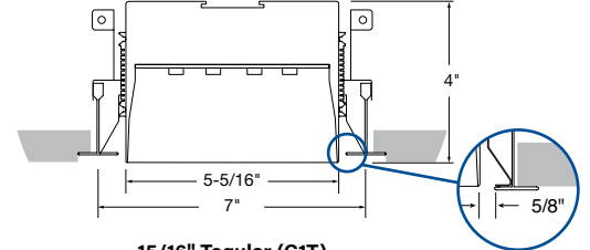
15/16" Tegular (C1T)
