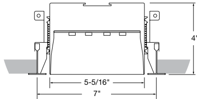
15/16" T-Bar (C1)
