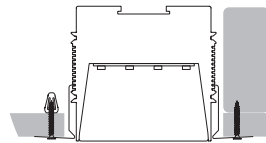
HP-4 WL SF
