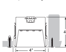
Recessed Spackle Flange
