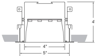
1" T-Bar (C1)
