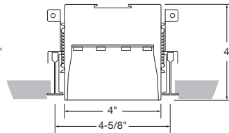
9/16" Tegular (C2T)
