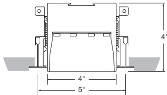
1" Tegular (C1T)
